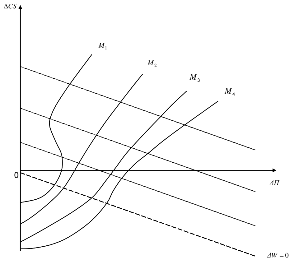
Figure 9: The merger curves in (\Delta\Pi, \Delta CS) -space. The downward-sloping lines are the iso-welfare curves.
